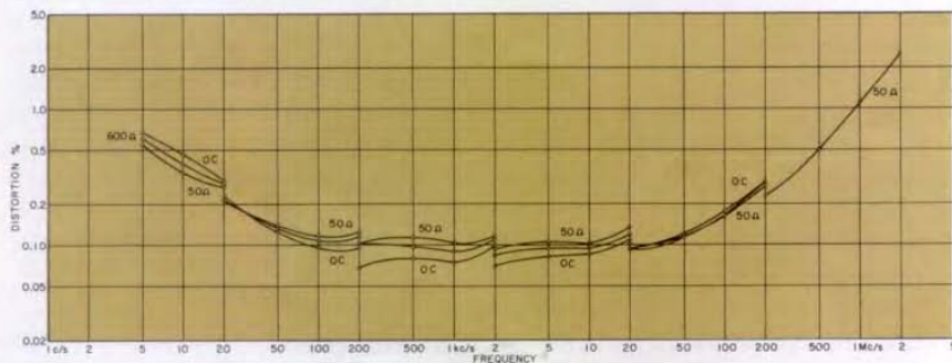
Figure 3. Measured harmonic distortion of a typical Type 1310-A Oscillator for 50-ohm and 600-ohm loads and open circuit. When the attenuator is used for open-circuit output voltages of five volts or less, the load seen by the oscillator is 600 ohms.
