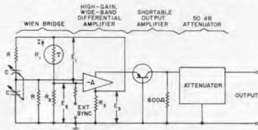
Figure 11. Simplified circuit diagram of Type 1310-A Oscillator.
