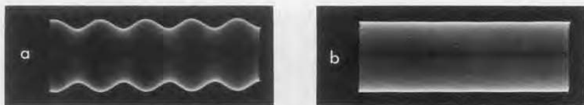
Figure 10. (a) 10-kc output of oscillator, amplitude modulated at 500 c/s by 9.5-kc signal fed into the synchronizing jack. (b) The reduction of the amplitude modulation in the output of an oscillator that has been locked to the a-m signal of (a).
