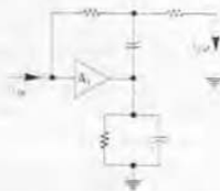
Figure 6. Functional diagram of a single section of the filter.
