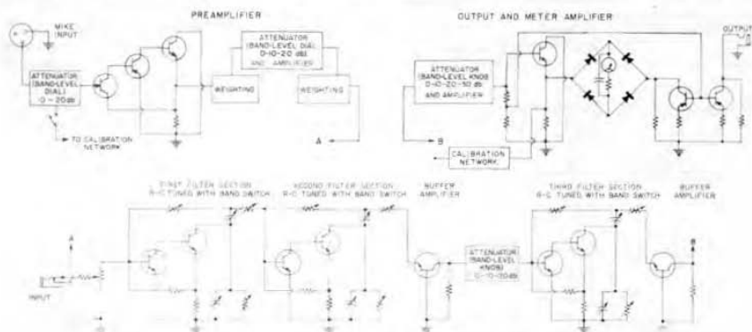
Figure 4. Schematic diagram of the Octave-Band Noise Analyzer.
