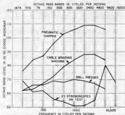
Figure 2. Typical octave-band pressure levels encountered in industry.
