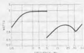
Figure 4. Typical output curves of the Type 1211-C Unit Oscillator.
