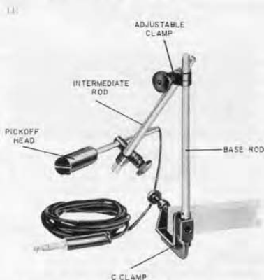
Figure 1. View of the Photoelectric Pickoff with component parts identified.
