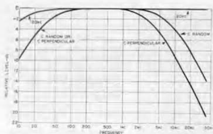
Figure 5. Frequency response characteristics of the preamplifier.
