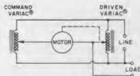
Figure 2. Elementary schematic of the servo system.
