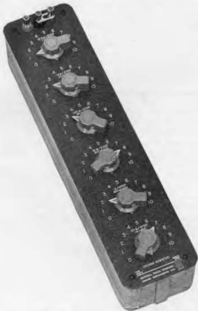
Figure 1. View of the Type 1432-X Decade Resistor.
