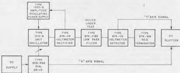
Figure 4. A typical setup for plotting frequency characteristics.
