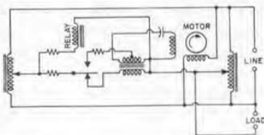
Figure 3. Schematic diagram showing the step-up transformer and protective relay.
