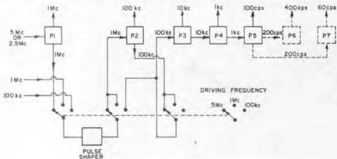
Figure 10. Block diagram of the Frequency Divider.
