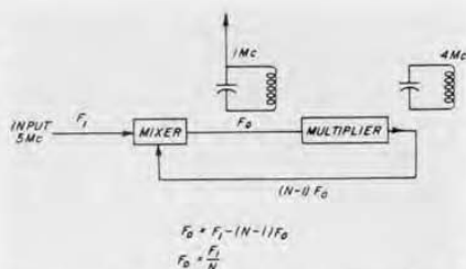
Figure 11. Elementary schematic of the 5:1 regenerative divider.
