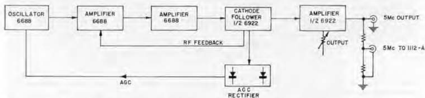
Figure 4. Block schematic of the Type 1113-A Standard-Frequency Oscillator.
