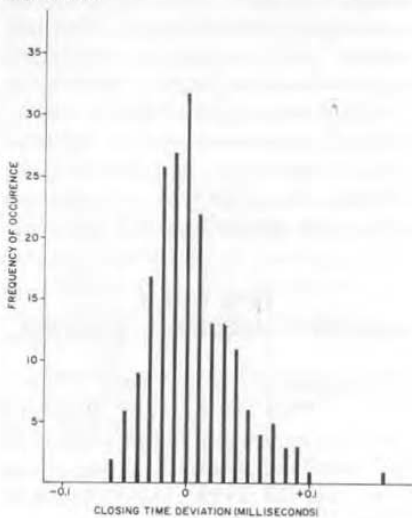
Figure 15. Histogram showing the random nature of variations in closure time of the contactor in the Type 1103-B Synchronometer. The average deviation is less than the average uncertainty in sky-wave reception of time signals.
