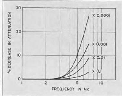
FIGURE 3. Frequency error in TYPE 700-P1 Voltage Divider.
