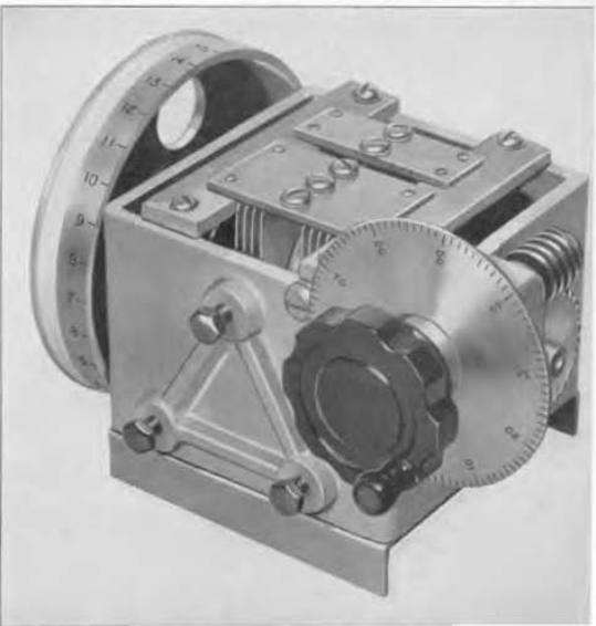
FIGURE 1. Low inductance, low losses, small size, and precision drive are some of the features of this condenser.
